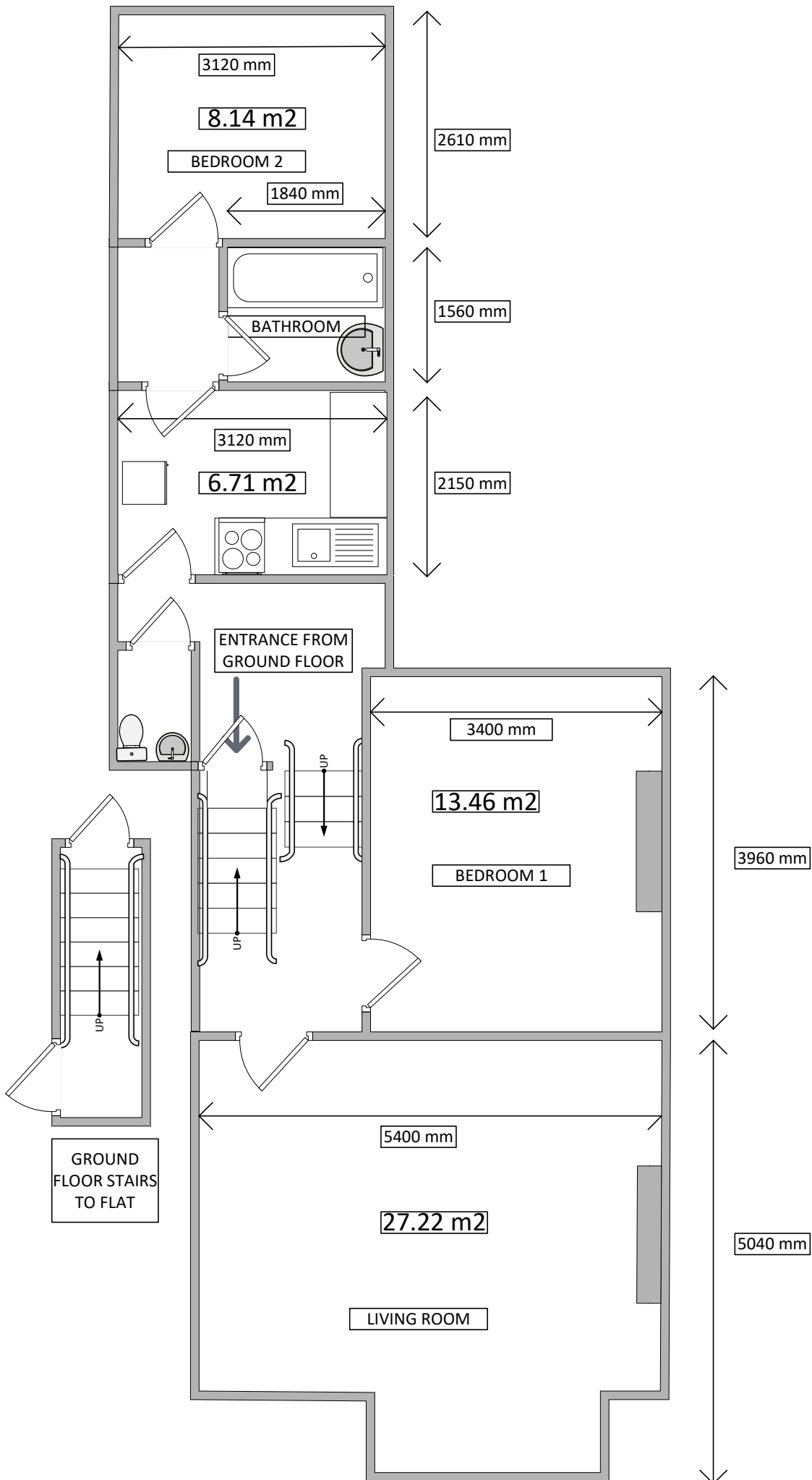
16 Barrington Road, N8 8QS – First Floor Plan
