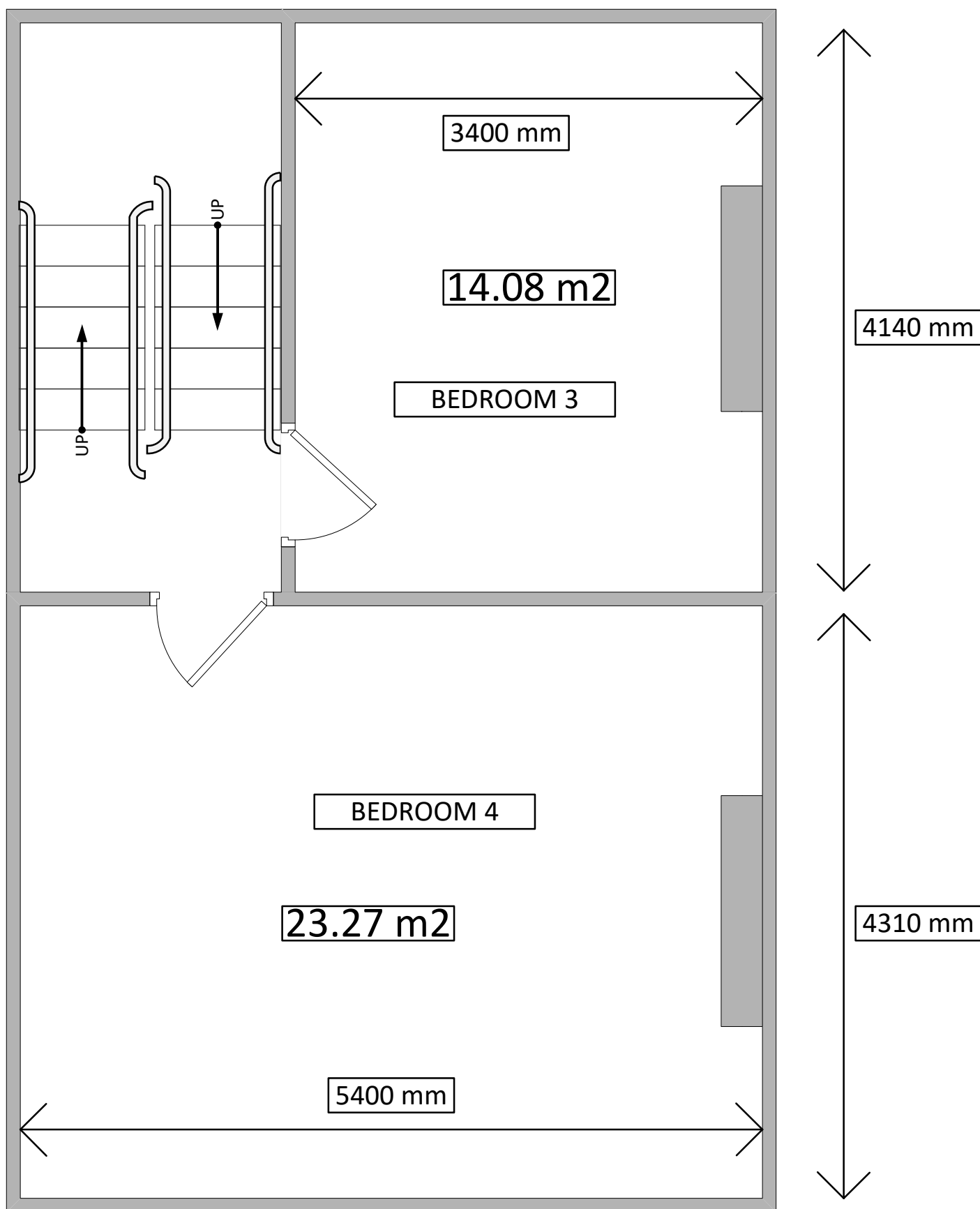
16 Barrington Road, N8 8QS Second Floor Plan
